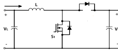
Gambar 4.1 Bidirectional DC-DC converter mode boost
